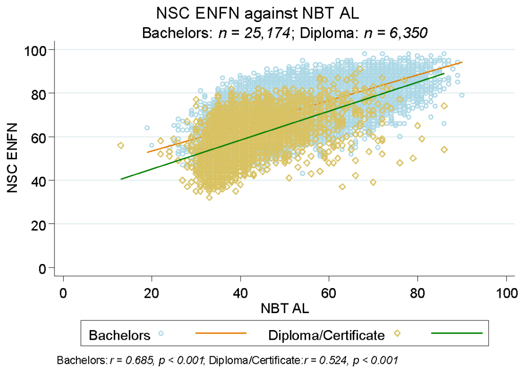
Figure 72 Scatterplot NBT AL vs NSC English First Additional Language
