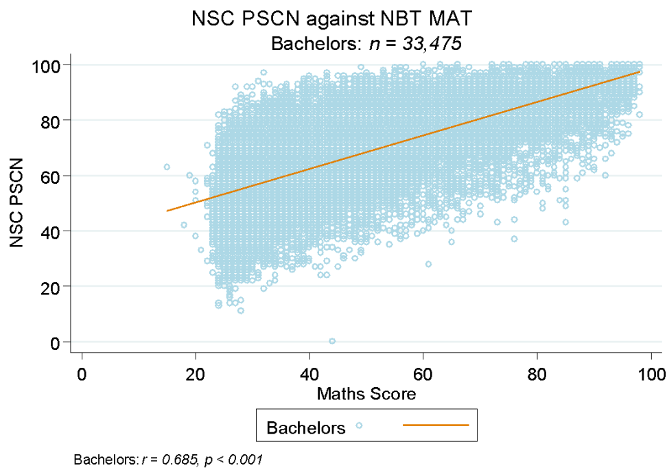
Figure 76 NSC PSCN vs NBT MAT
