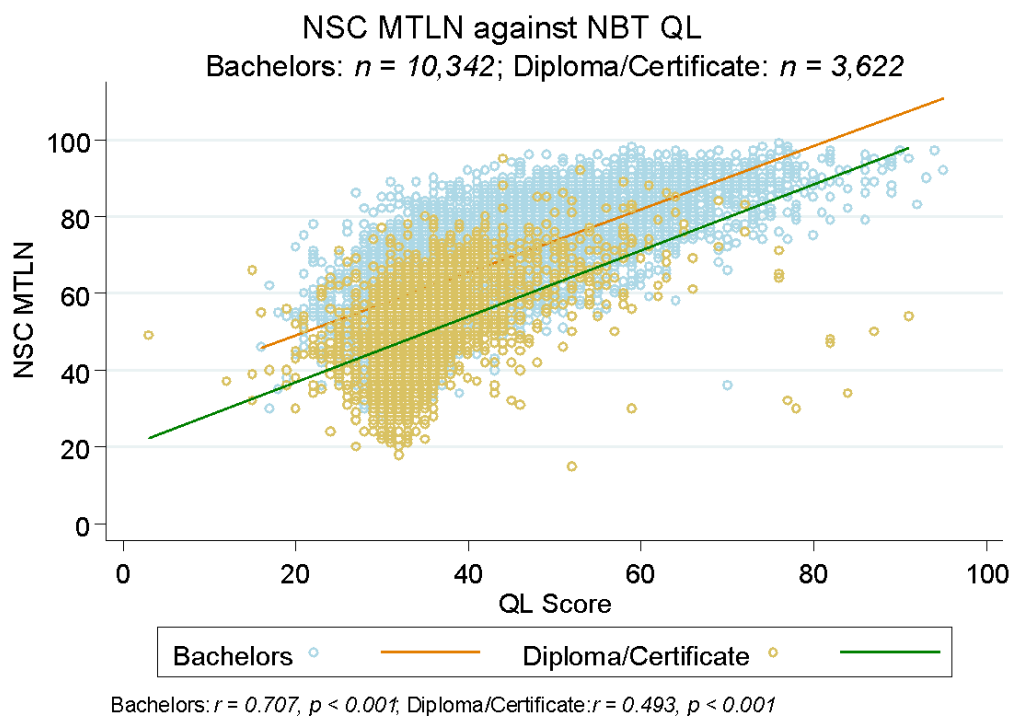
Figure 74 Scatterplot NBT QL vs NSC mathematical Literacy
